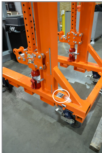
RBJ20K LOCATION
