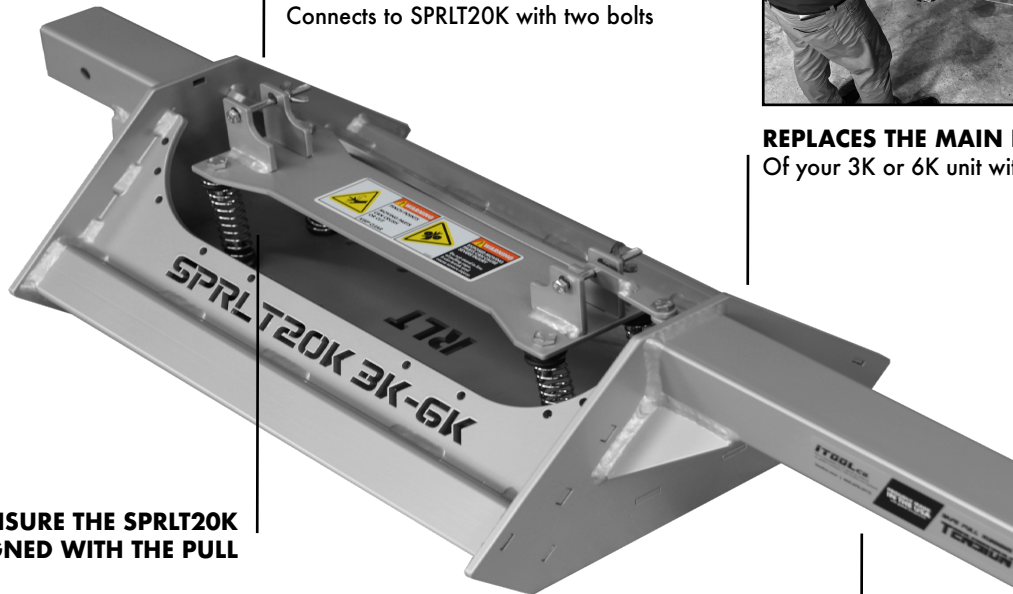
CARRIAGE FOR RUNNING LINE TENSION METER Connects to SPRLT20K with two bolts
