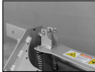
CARRIAGE FOR RUNNING LINE TENSION METER Connects to SPRLT20K with two bolts
