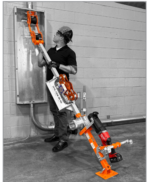
Works in Overhead, Underground & Side Pull Applications
