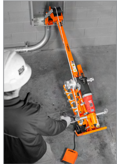
Dual Capstans
